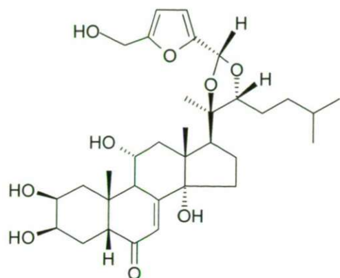
serfurosterone B (17)*
