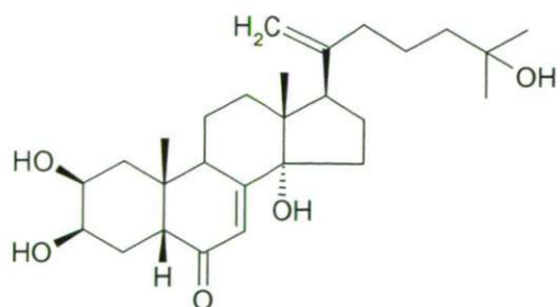
22-deoxy-20,21-didehydro-ecdysone (23)*
