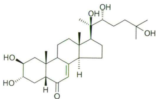
2 \beta ,3 \alpha ,20R,22R,25-pentahydroxy-5 \beta -14 \alpha -cholest-7-en-6-one (3)*
