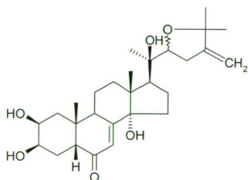
24-methylene-shidasterone (15)*
