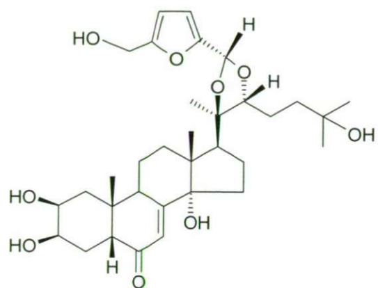
serfurosterone A (9)*
