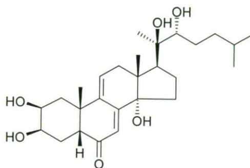
2 \beta ,3 \alpha ,20R,22R,25-pentahydroxy-5 \beta -14 \alpha -cholest-7-en-6-one (3)*
