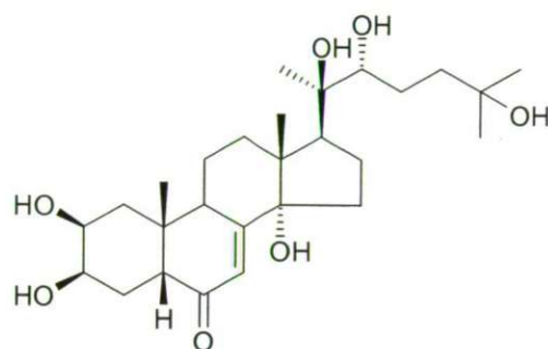
20-hydroxyecdysone (11)
