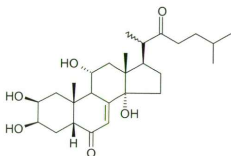
22-dehydro-20-deoxy-ajugasterone C (19)*
