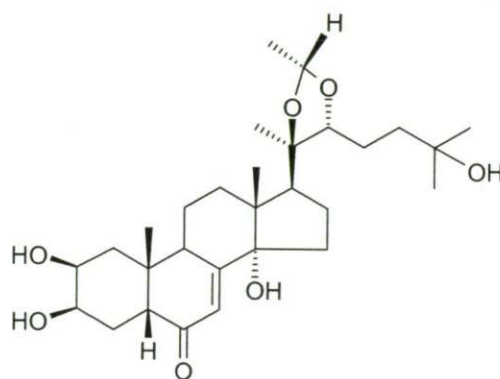
1-hydroxy-20,22-didehydrotaxisterone (18)*
