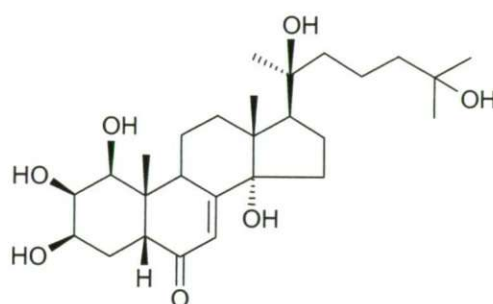
22-deoxyintegristerone A (12)
