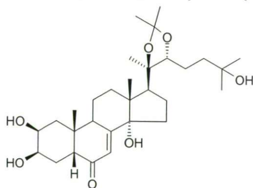
20-hydroxyecdysone 20,22-ethylidene (20)
