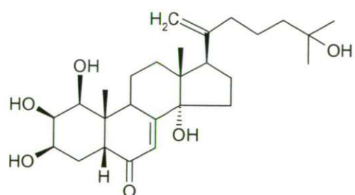
1-hydroxy-22-deoxy-20,21-didehydro-ecdysone (21)*
