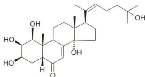
1-hydroxy-20,22-didehydrotaxisterone (18)*
