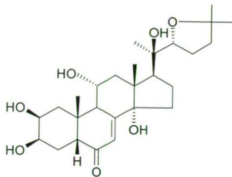
11 \alpha -hydroxyshidasterone (1)*
