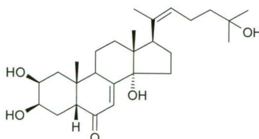
20,22-didehydrotaxisterone (16)*
