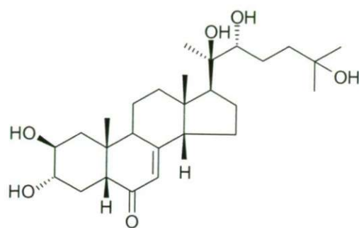
2 \beta ,3 \alpha ,20R,22R,25-pentahydroxy-5 \beta -14 \beta -cholest-7-en-6-one (2)*
