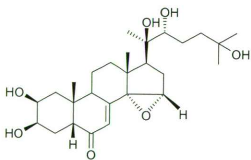
14 \alpha ,15 \alpha -epoxy-14,15-dihydrostachysterone B (7)*
