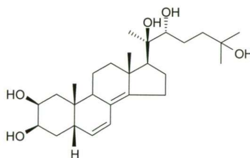
2β,3β,20R,22R,25-pentahydroxy-5β-cholest-6,8(14)-diene (14)*
