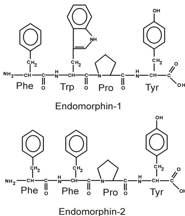
Fig. 1. Chemical structure of the EMs
