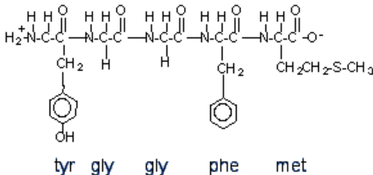
Fig. 2. Chemical structure of Met-enkephalin
