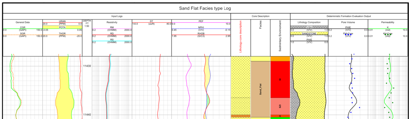
Fig. 2-5 Sand Flat Facies Log Response
