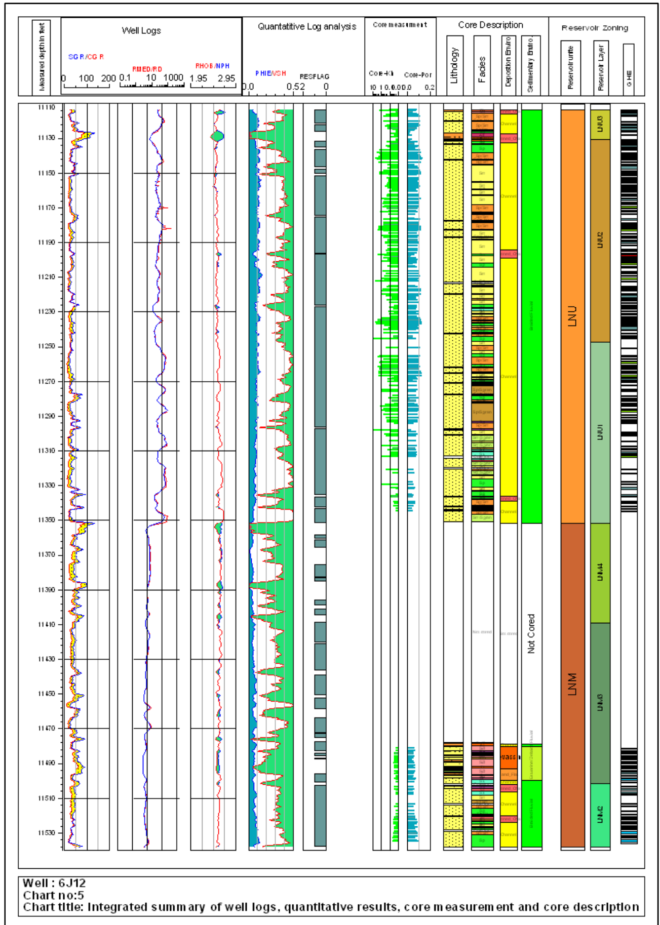
Fig. 1-5 Integrated Interpretation Chart Well: 6J12
