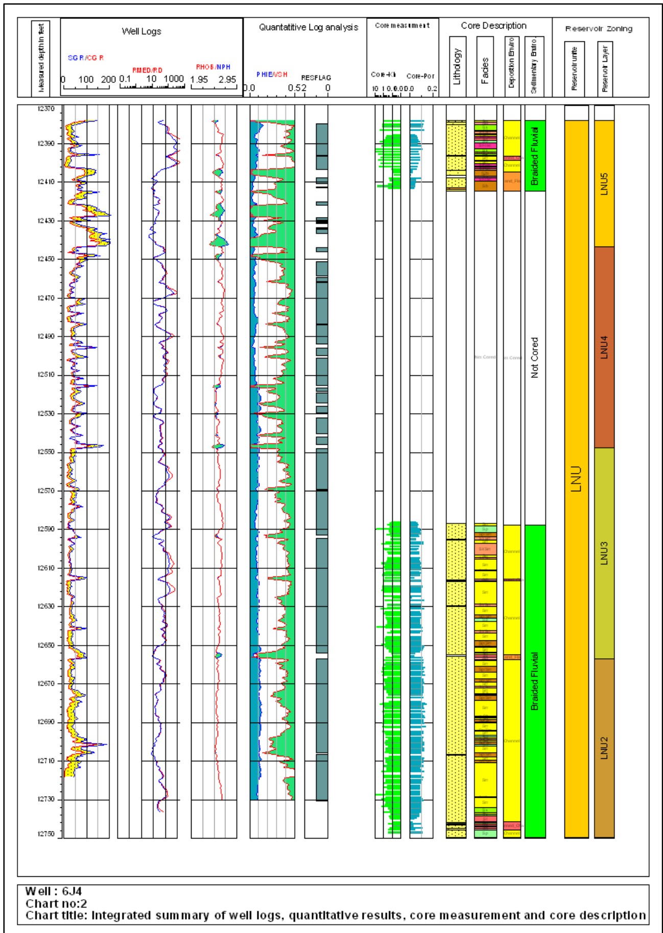
Fig. 1-2 Integrated Interpretation Chart Well: 6J4
