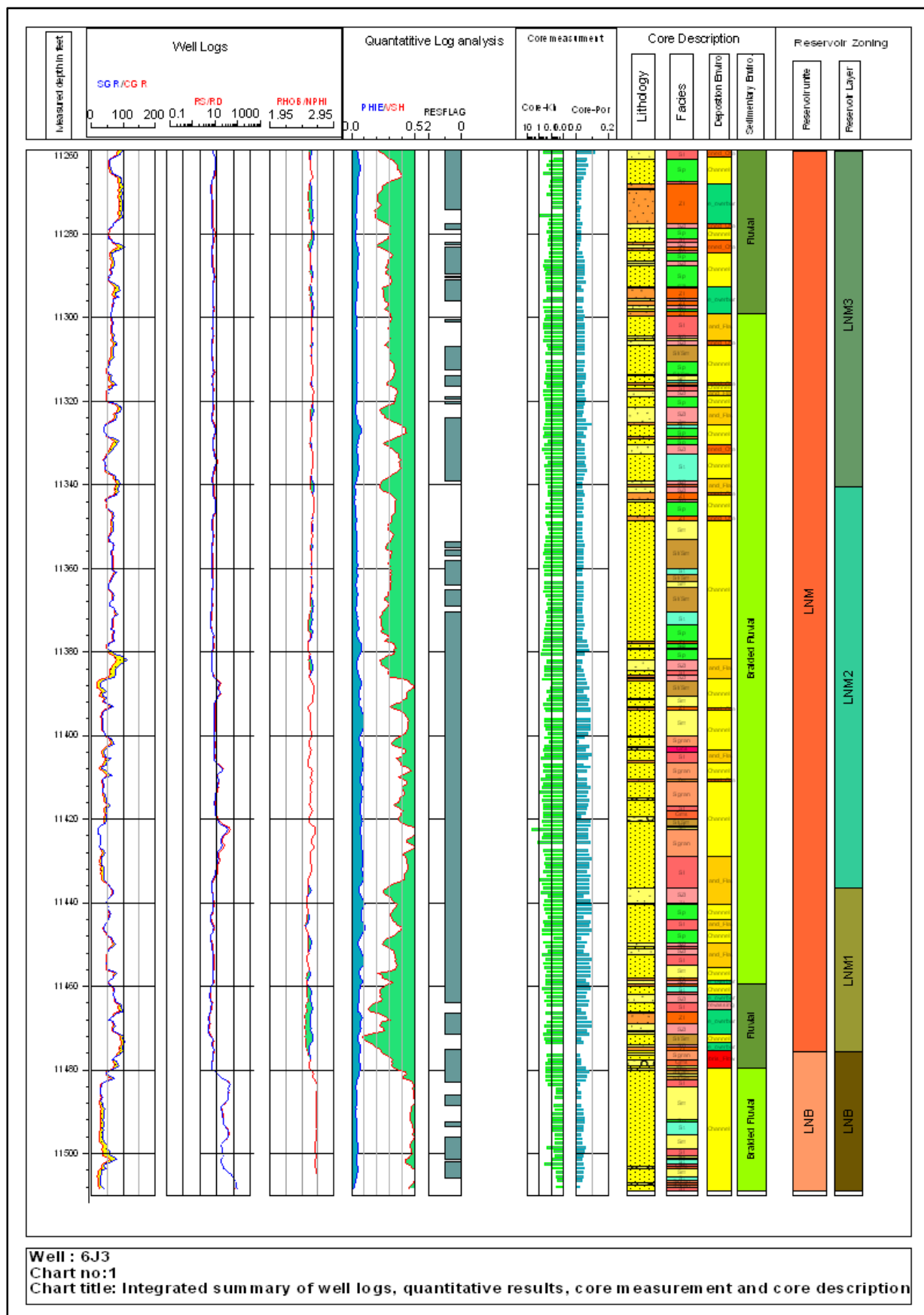
Fig. 1-1 Integrated Interpretation Chart Well: 6J3
