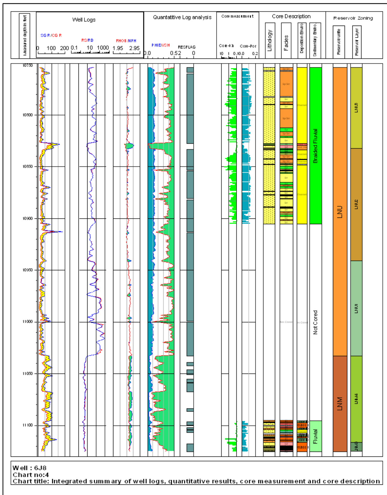
Fig. 1-4 Integrated Interpretation Chart Well: 6J8
