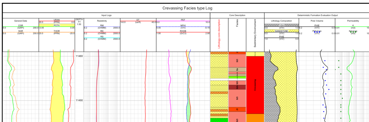
Fig. 2-3 Crevassing Facies Log Response
