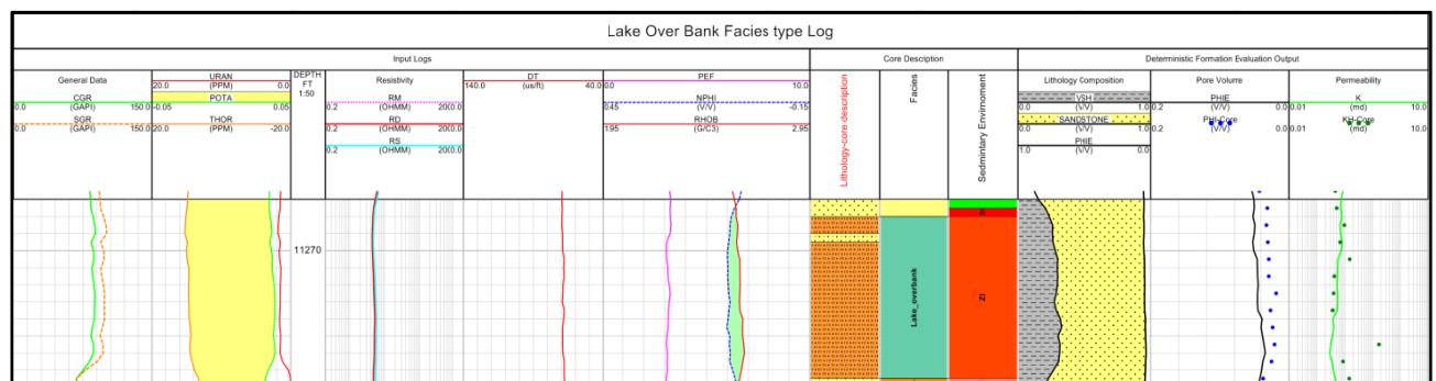
Fig. 2-7 Lake Over Bank Facies Log Response
