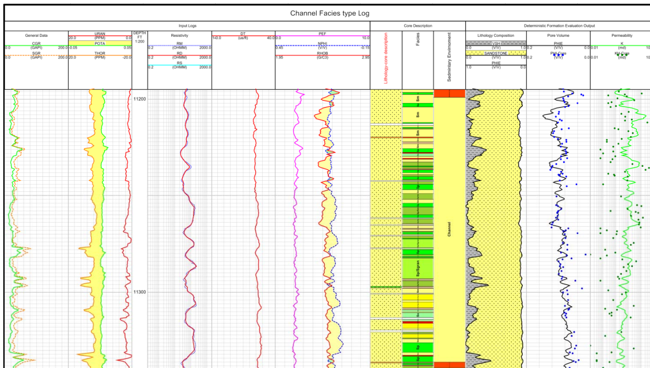
Fig. 2-1 Channel Facies Log Response
