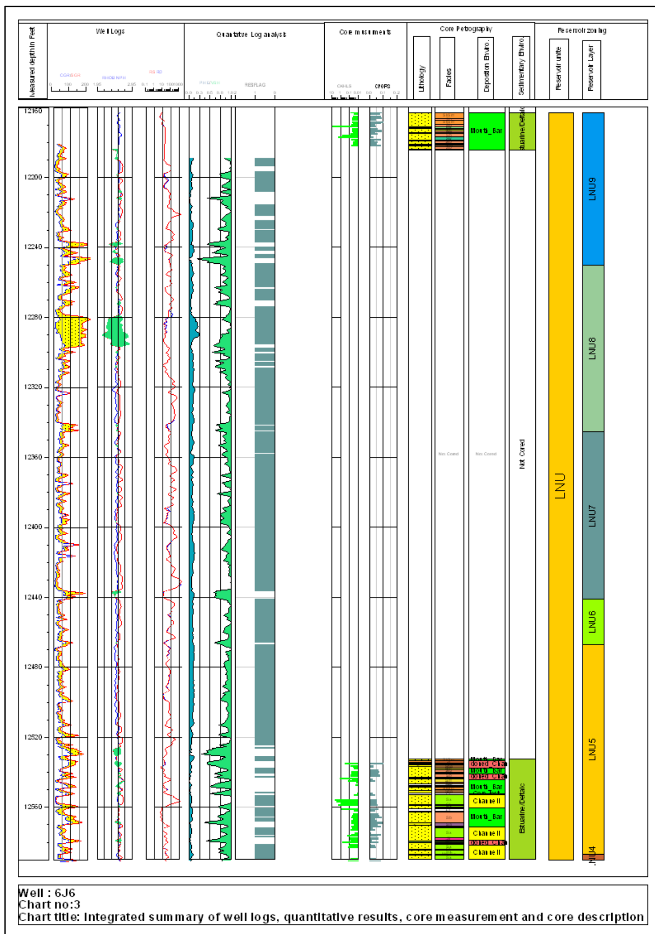
Fig. 1-3 Integrated Interpretation Chart Well: 6J6
