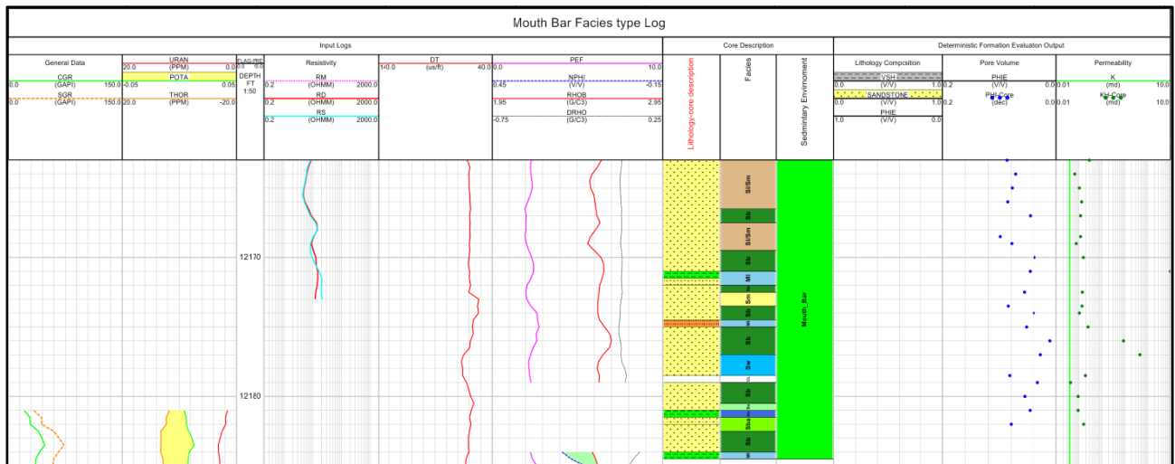
Fig. 2-4 Mouth Bar Facies Log Response
