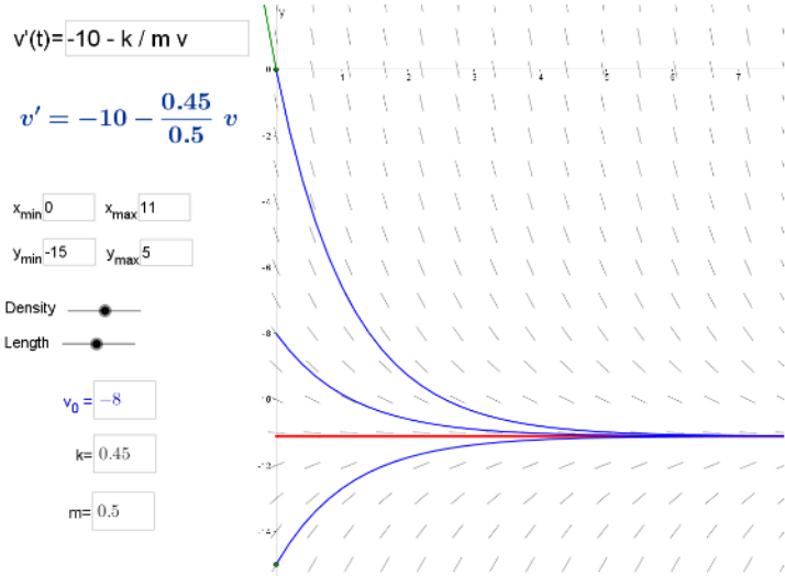
Figure 13. Skydiving analysis (GeoGebra [8])
