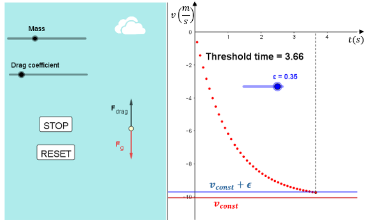
Figure 14. The ice ball v(t) , GeoGebra [1] function
