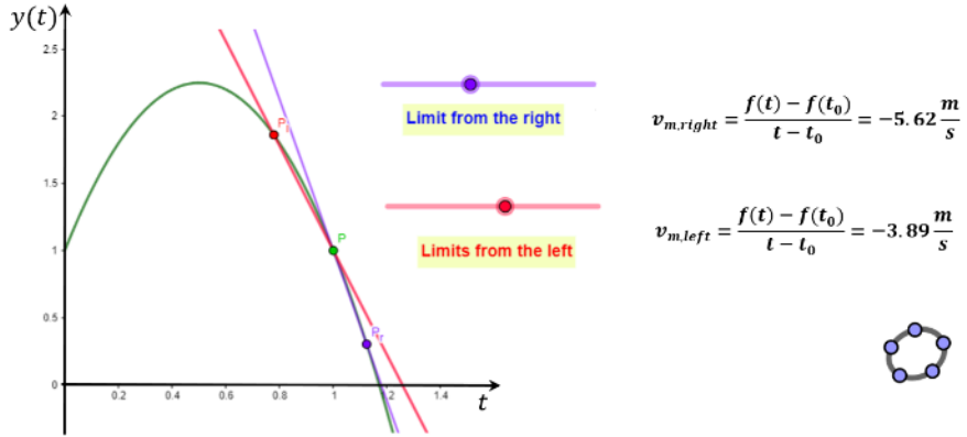
Figure 3. Approximations of instantaneous velocity (GeoGebra [3])
